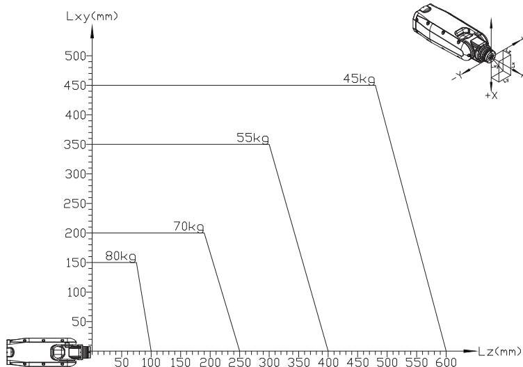
Robot payload diagram
