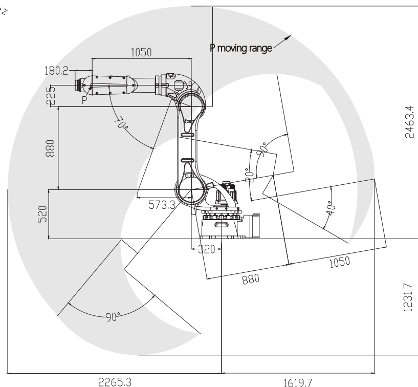
P moving range
