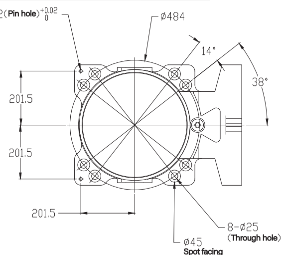
Base installation dimensions
