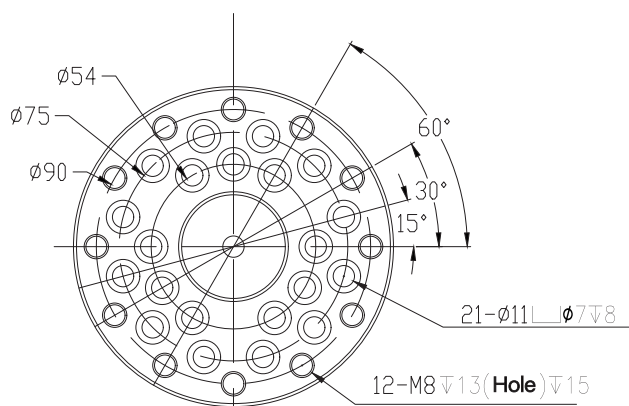
End flange installation dimensions
