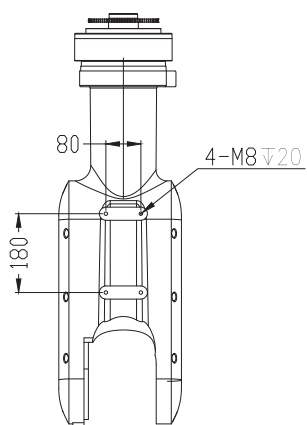
Wrist installation dimensions
